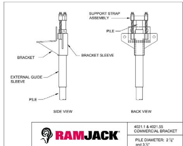
FIGURE 5—4021.1 SUPPORT BRACKET ASSEMBLY WITH GUIDE SLEEVE AND PILING
